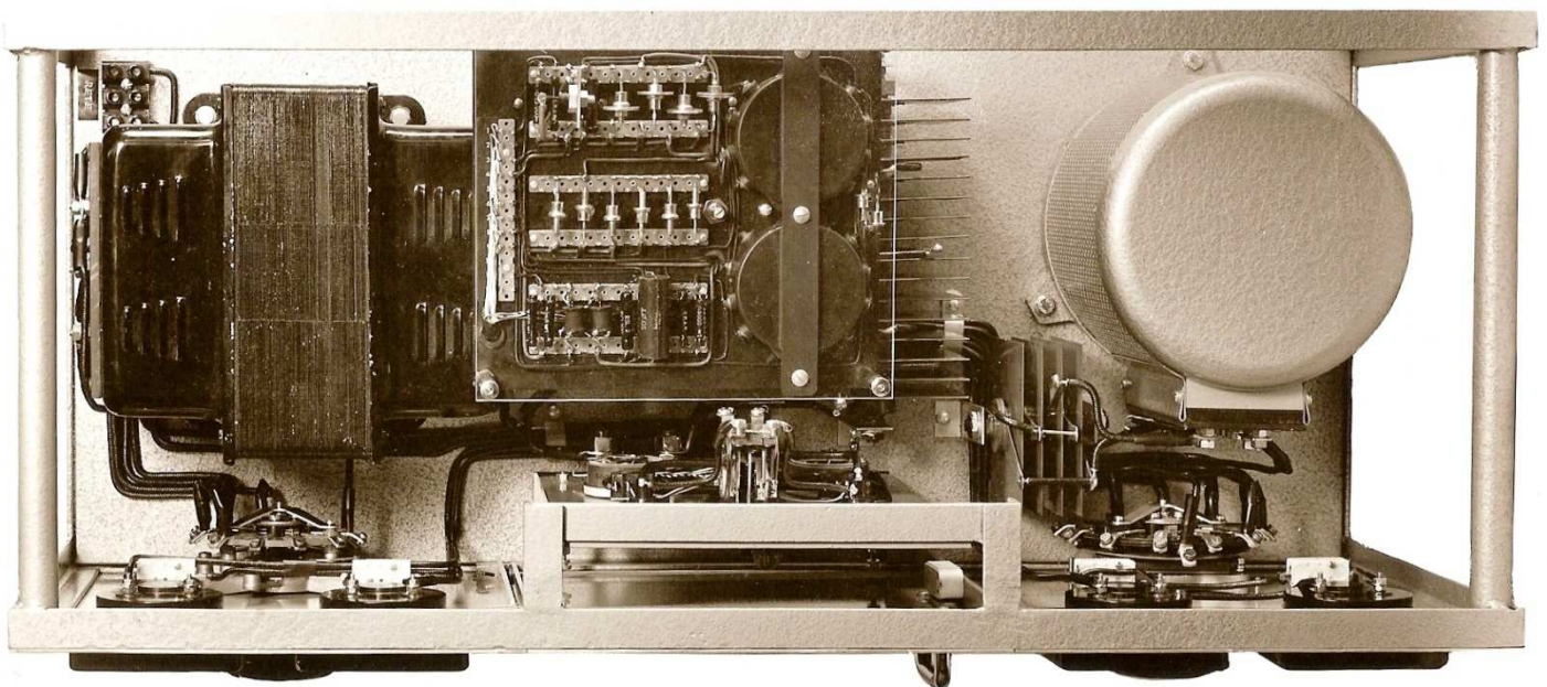
Automatic T-R unit mod. 236-17
